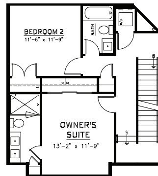
THIRD FLOOR ALTERNATE PLAN
